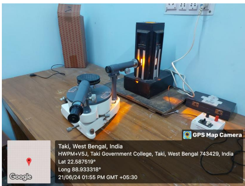
Spectrometer and Sodium Vapour Lamp
